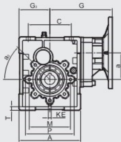
BKM..IEC外形尺寸 / Outline Dimension
